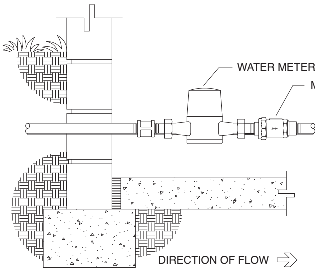
INDOOR INSTALLATION
