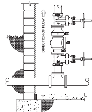
VERTICAL INSTALLATION (350OSYG)
