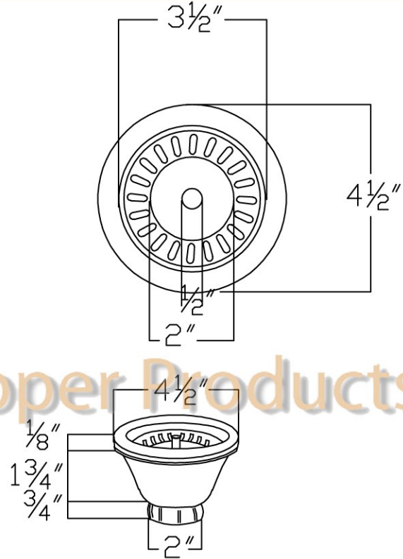
D-132ORB STRAINER DRAIN SHOWN BELOW
